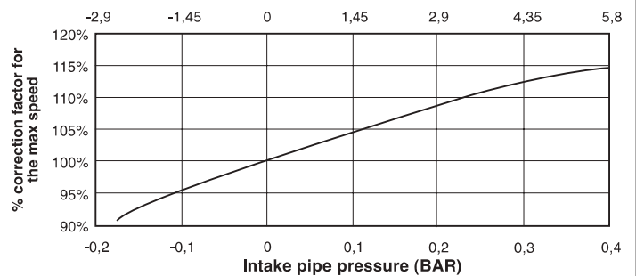
max speed / intake pipe pressure
