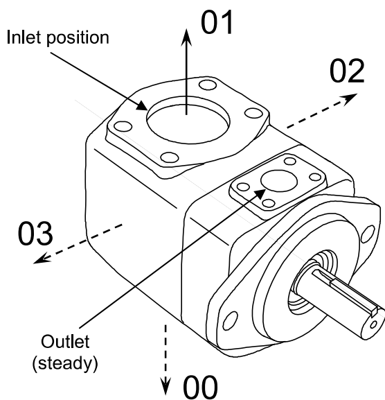
Port orientations
