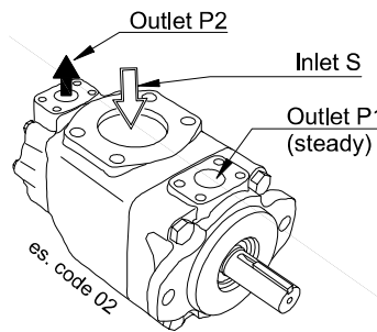
Port orientations
